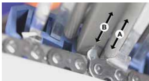
Sharpening of cutting tooth (A) and adjustment of depth gauge (B) in a one-step operation
