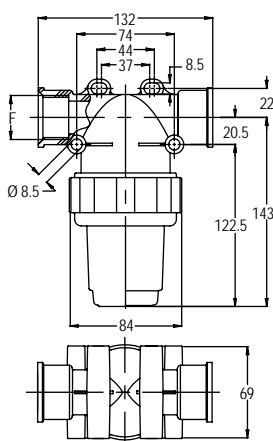
G 1"
