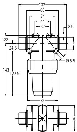
G 1"
